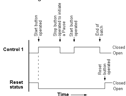
Fig 7 Reset status timing
