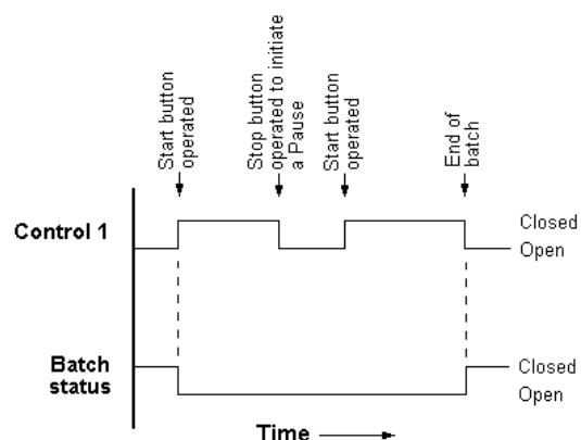
Fig 8 Batch status timing
