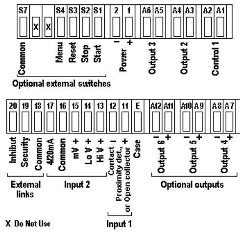
Fig 5 Dimensions and terminal connections
