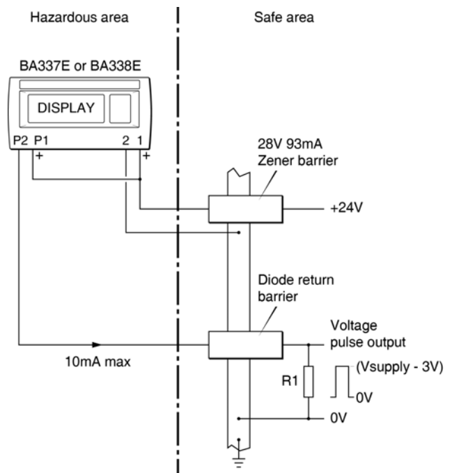
Fig 17 Transferring pulse output to the safe area using Zener barriers
