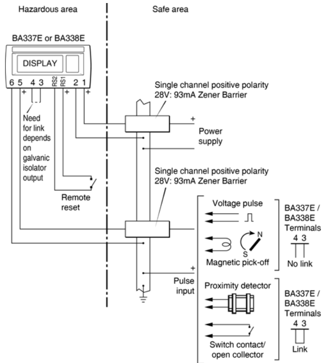
Fig 3 BA337E or BA338E used with Zener barriers pulse source in safe area.
