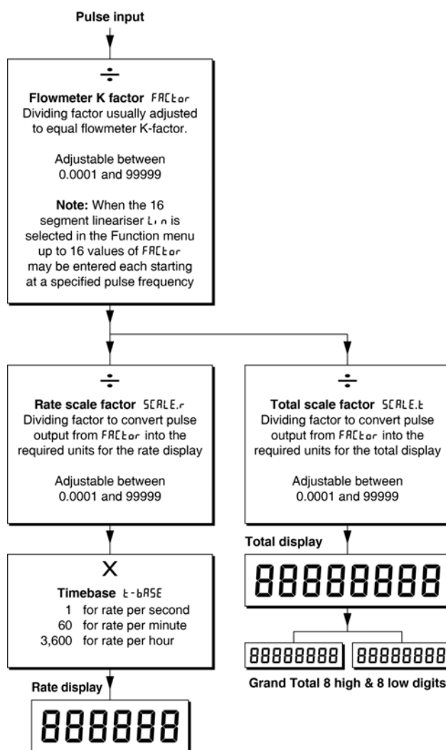
Fig 9 Calibration structure
