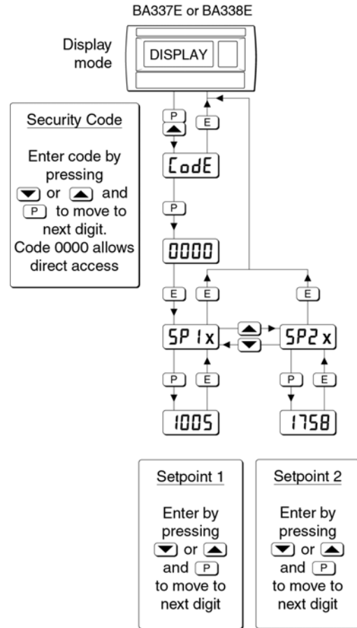
Fig 16 Setpoint adjustment from the totalisation mode
