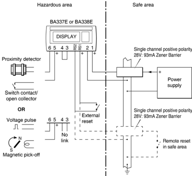
Fig 2 BA337E or BA338E used with Zener barriers
