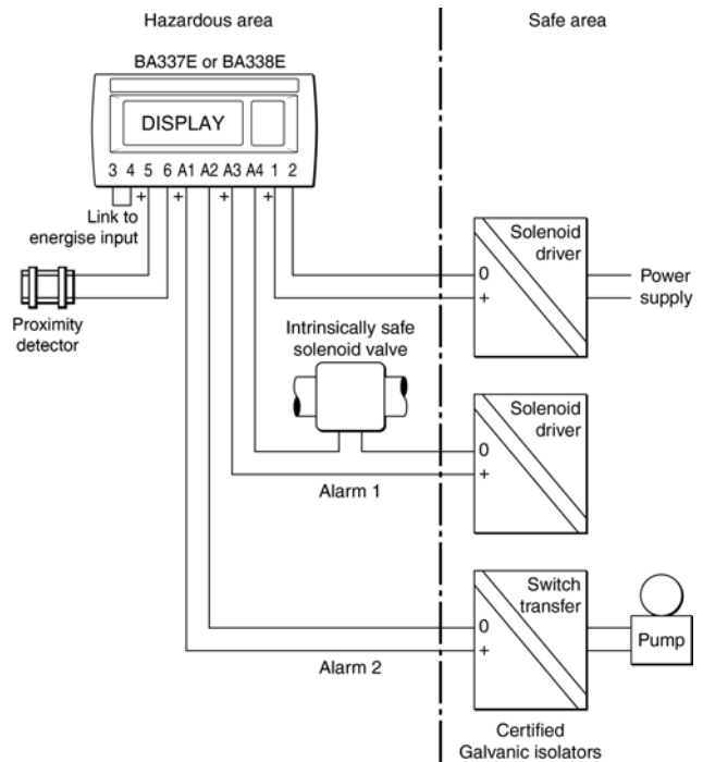
Fig 14 Typical alarm application
