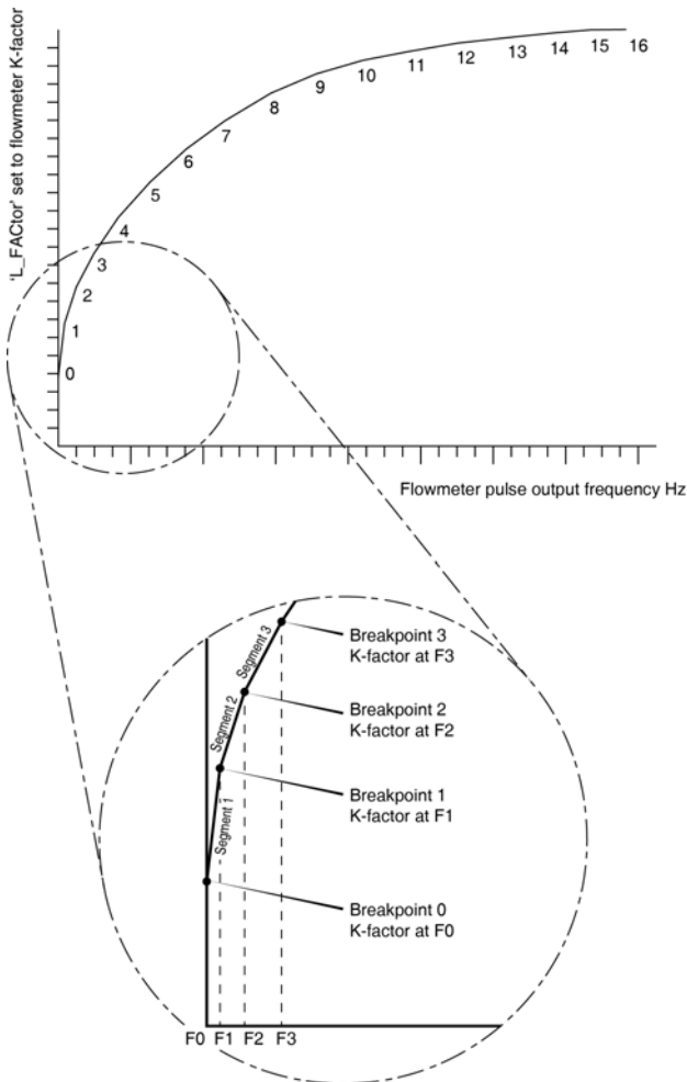
Fig 11 shows a typical linearising characteristic
