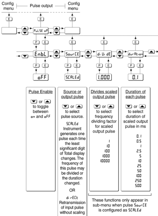
Fig 18 Pulse output configuration sub-menu
