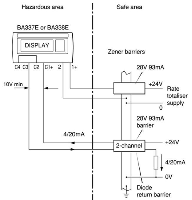
Fig 19 Application of 4/20mA output
