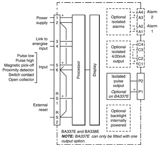
Fig 1 BA337E and BA338E block diagram
