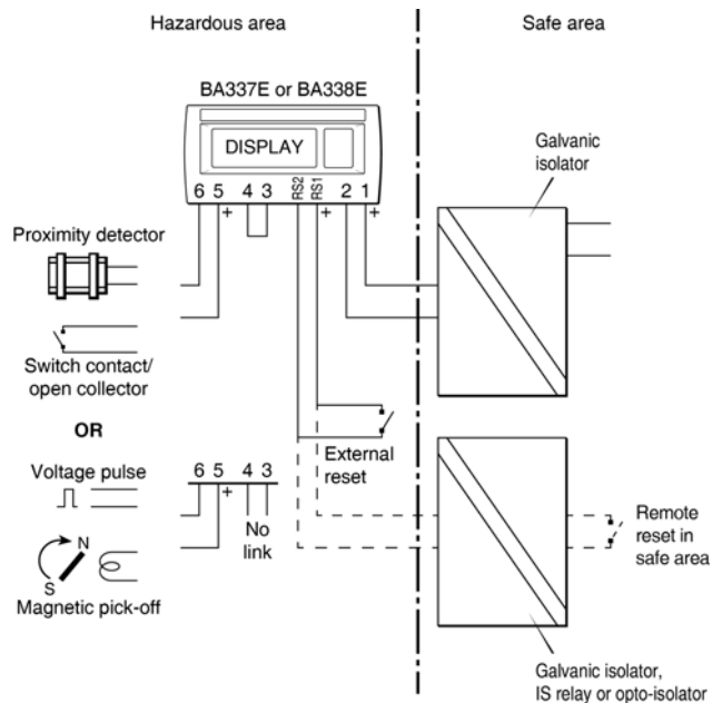
Fig 4 BA337E or BA338E used with galvanic isolators.
