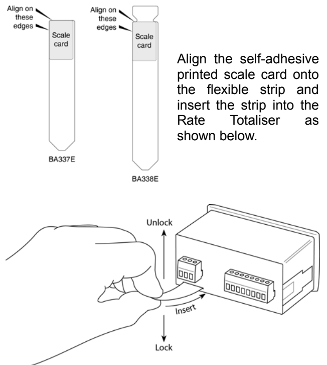
Fig 8 Inserting the flexible strip carrying the scale card into slot at the rear of Rate Totaliser.
