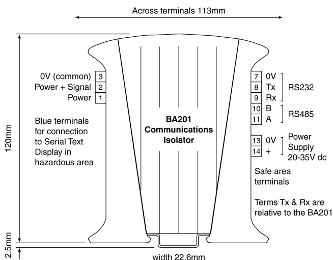
Fig 1 BA201 dimensions and terminal numbers
