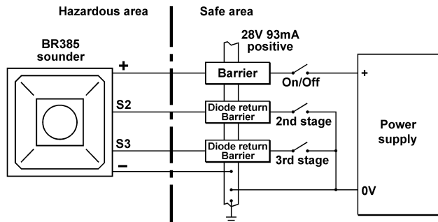
Fig 6 Multi-stage alarm using Zener barriers.
