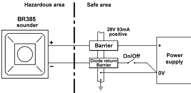
Fig 5 Single stage alarm using two channel barrier.
